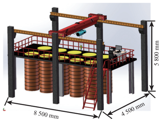
图4 用于修正测井方法的全尺寸固井水泥环模拟井群 Fig.4 Full-size cementing ring simulation of a well cluster for modified logging methods
